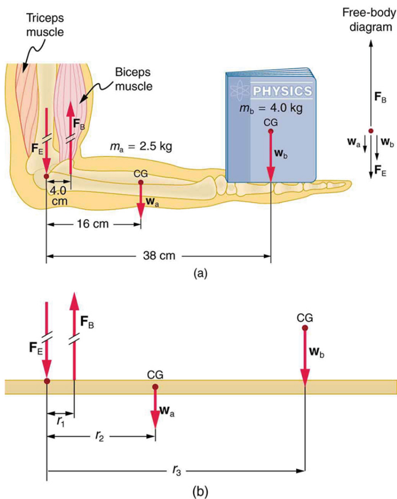
Figure 9.26 (a) The figure shows the forearm of a person holding a book. The biceps exert a force F_B to support the weight of the forearm and the book. The triceps are assumed to be relaxed. (b) Here, you can view an approximately equivalent mechanical system with the pivot at the elbow joint as seen in Example 9.4 .
